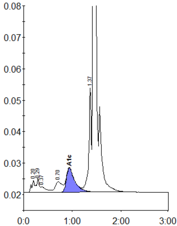
Peak table - ID: 10649196
